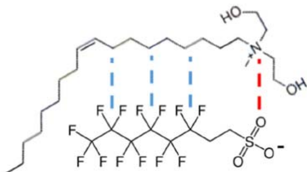
Figure 19. The interaction between the PFAS molecule (below shown for the example of 6:2 FTS) and the added cation (taken from Maga et al 2021)
