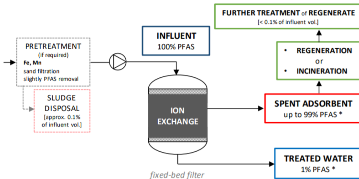
Figure 17. PFAS flow diagram for adsorption filtration with IEX /taken from (Concawe, 2020)).
