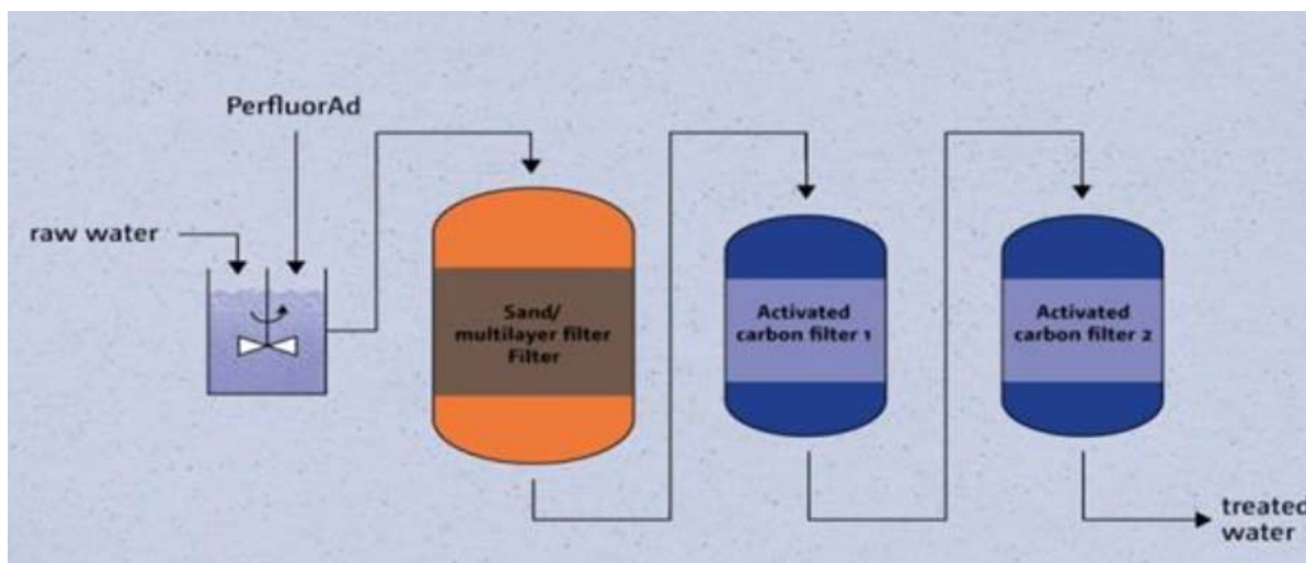
Figure 18. Schematic overview of an Activated Carbon Plant (GAC) with PerfluorAd Pre-treatment Stage (taken from Cornelsen)
