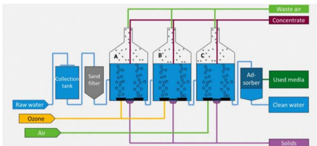
Figure 22. Ozofractionation process concept (taken from (UBA, 2020)).
