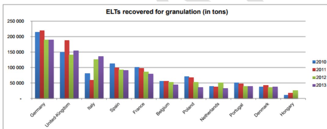
Figure A 5: ELTs recovered for granulation (in tonnes)
