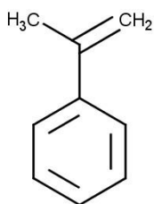
2-phenylpropene
