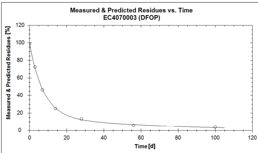
Figure 28: Residuals of EC 407-000-3 vs. time in the whole system of an aerobic river – DFOP.
