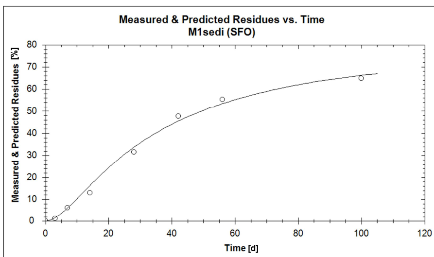
Figure 67: Measured and predicted residues of M1 vs. time in the sediment phase of an anaerobic pond – SFO.
