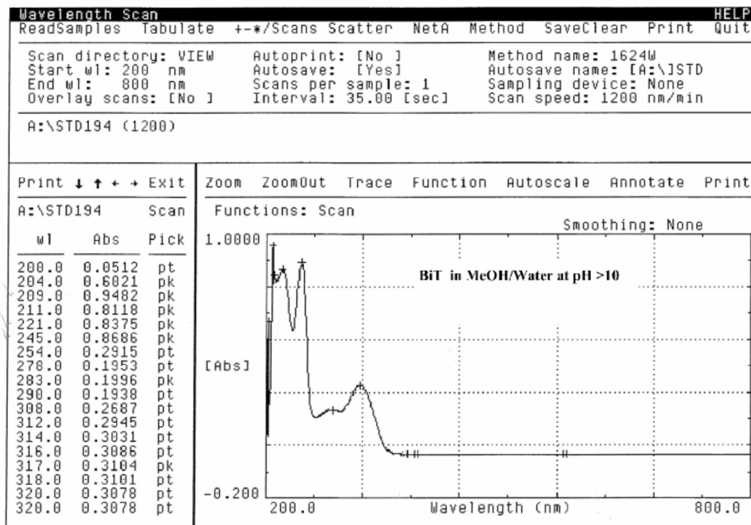
Figure A7.1.1.1.2/2-3: UV/Visible spectra of 1,2-benzisothiazolin-3-one at pH > 10
