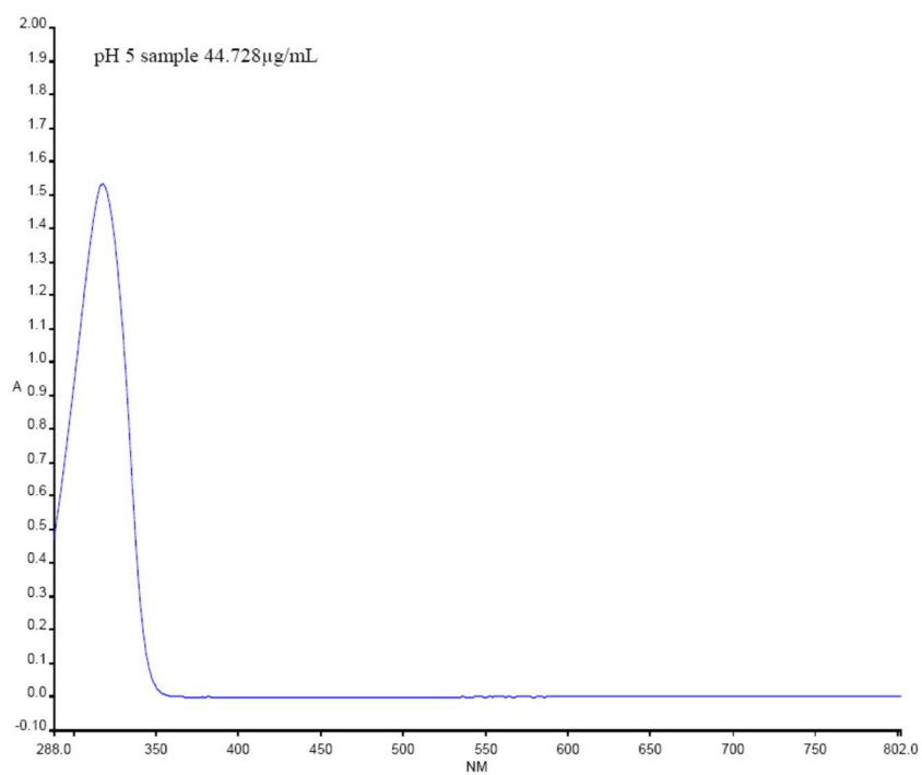
Figure A7.1.1.1.2/1-1: UV-VIS absorption spectrum of BIT in pH 5 buffer solution
