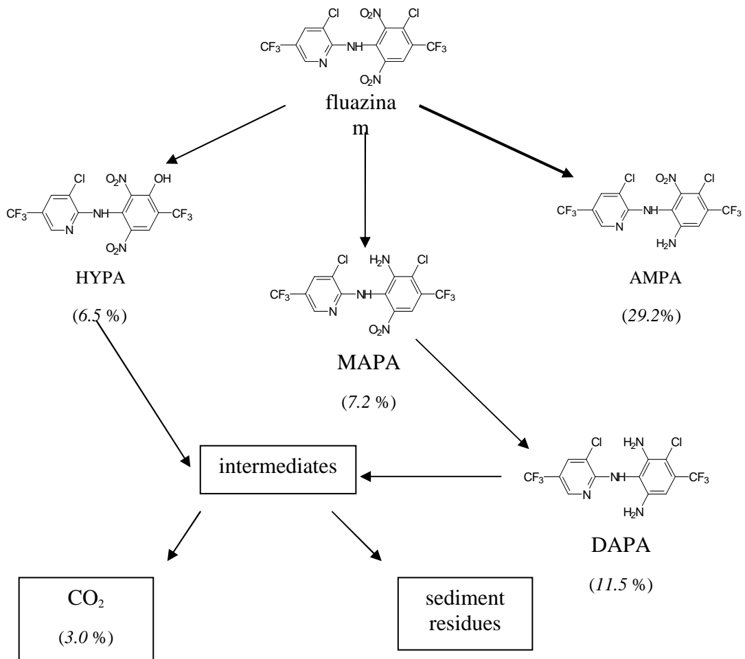
Proposed metabolic pathway of fluazinam in water/sediment systems (values in bracket: maxima observed in the whole system for a single label position)
