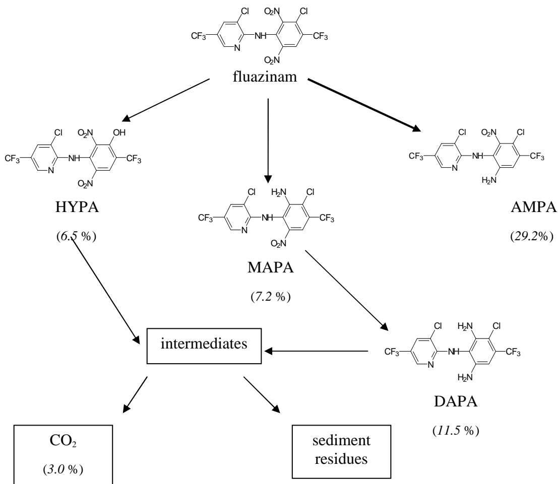
Proposed metabolic pathway of fluazinam in water/sediment systems (values in brackets: maxima observed in the whole system for a single label position)
