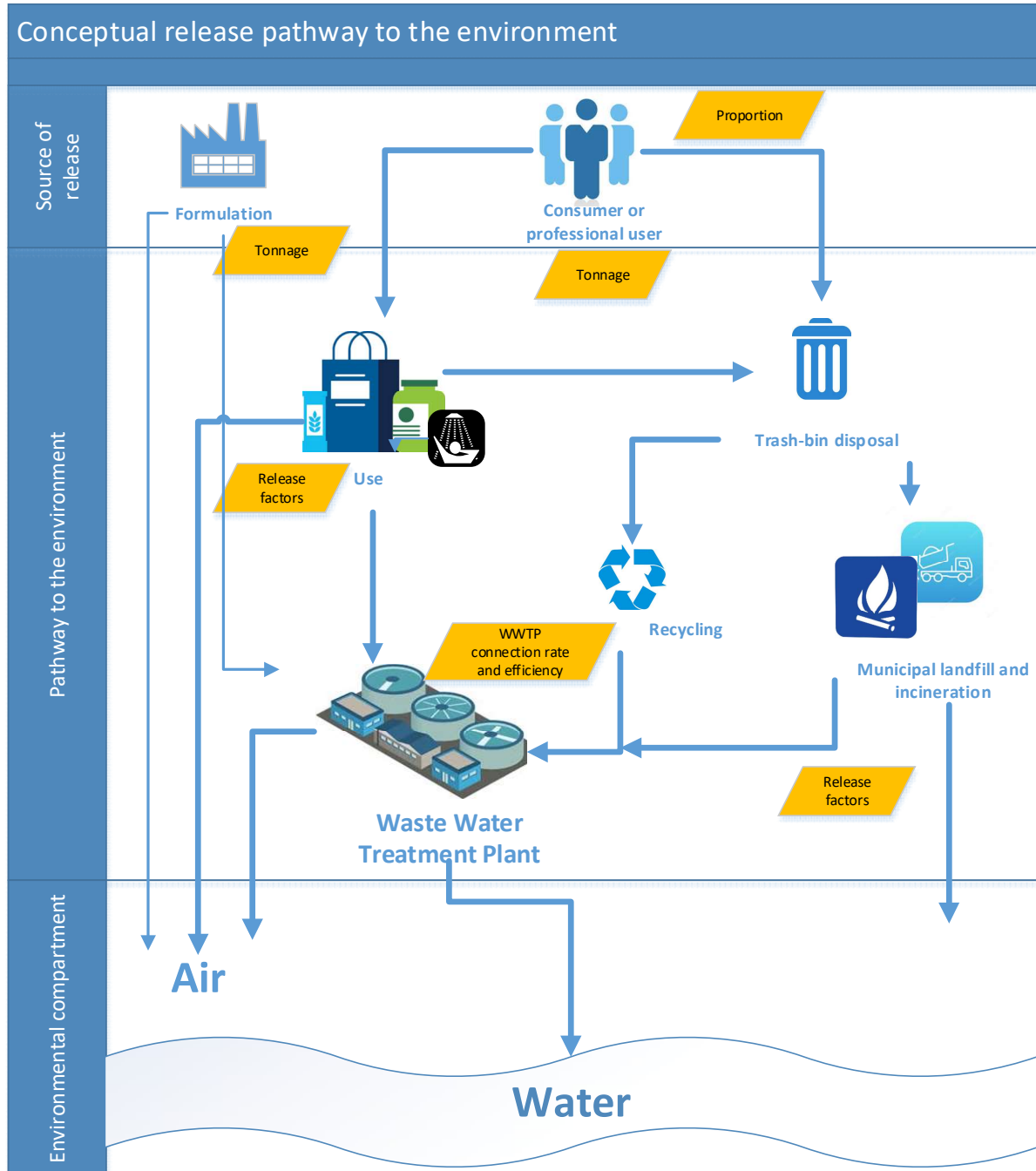
Figure 4: Conceptual source, pathway, receptor relationships for uses of D4, D5 and D6
